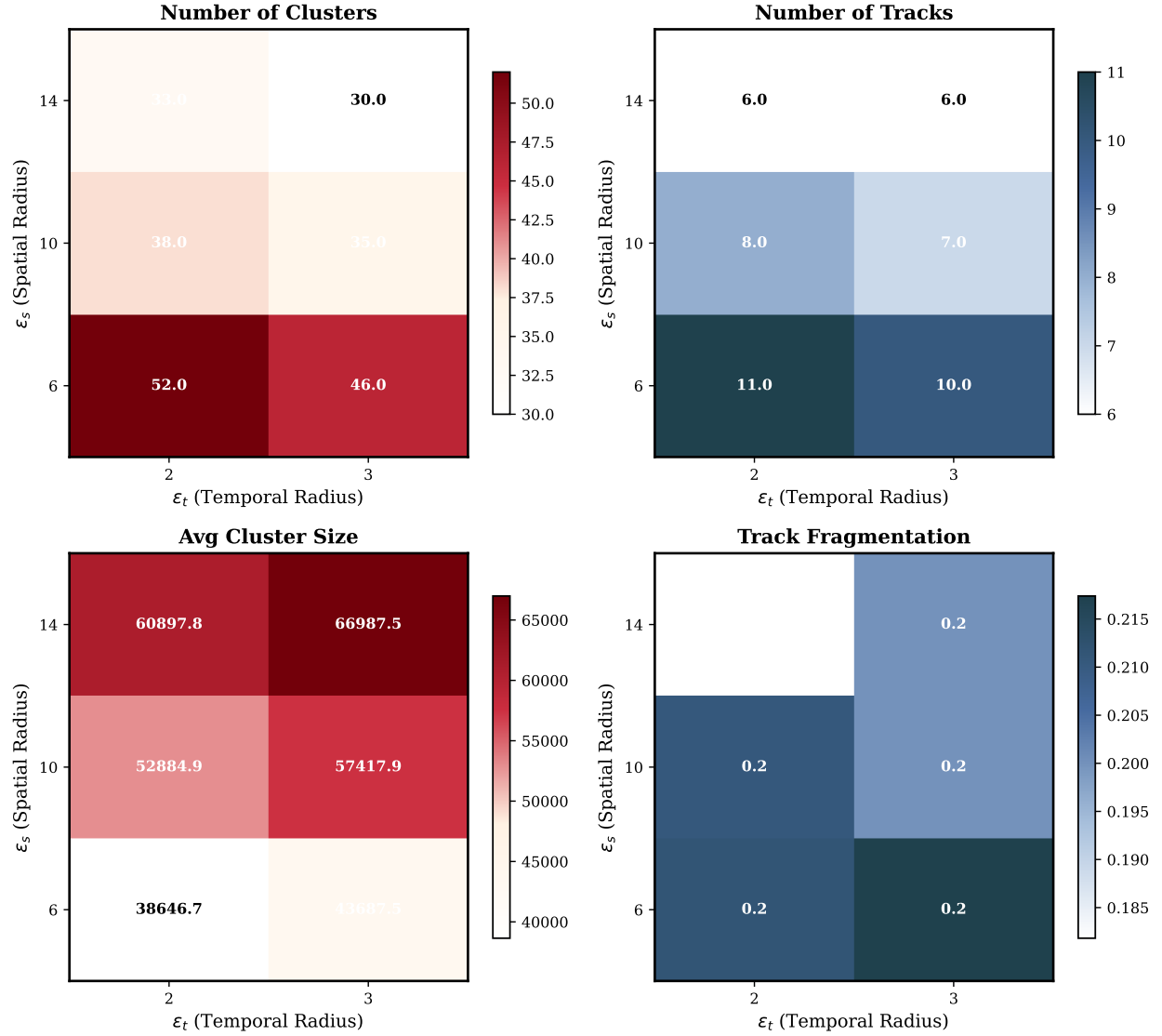
Fig. 14 Parameter interaction heatmaps showing the combined effect of spatial radius \epsilon_s and temporal radius \epsilon_t on clustering and tracking metrics.
