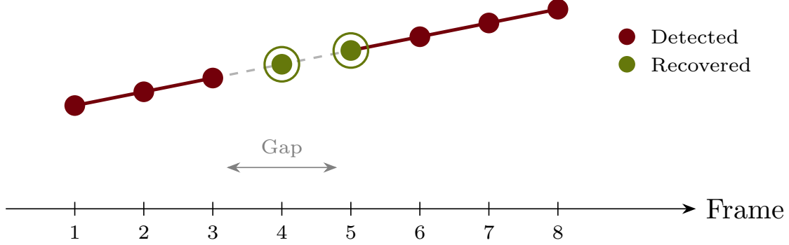
Fig. 3 Gap recovery mechanism. When a vessel temporarily disappears (frames t_1 to t_2 ), the algorithm reconnects clusters based on centroid proximity, maintaining track identity across brief dropouts.
