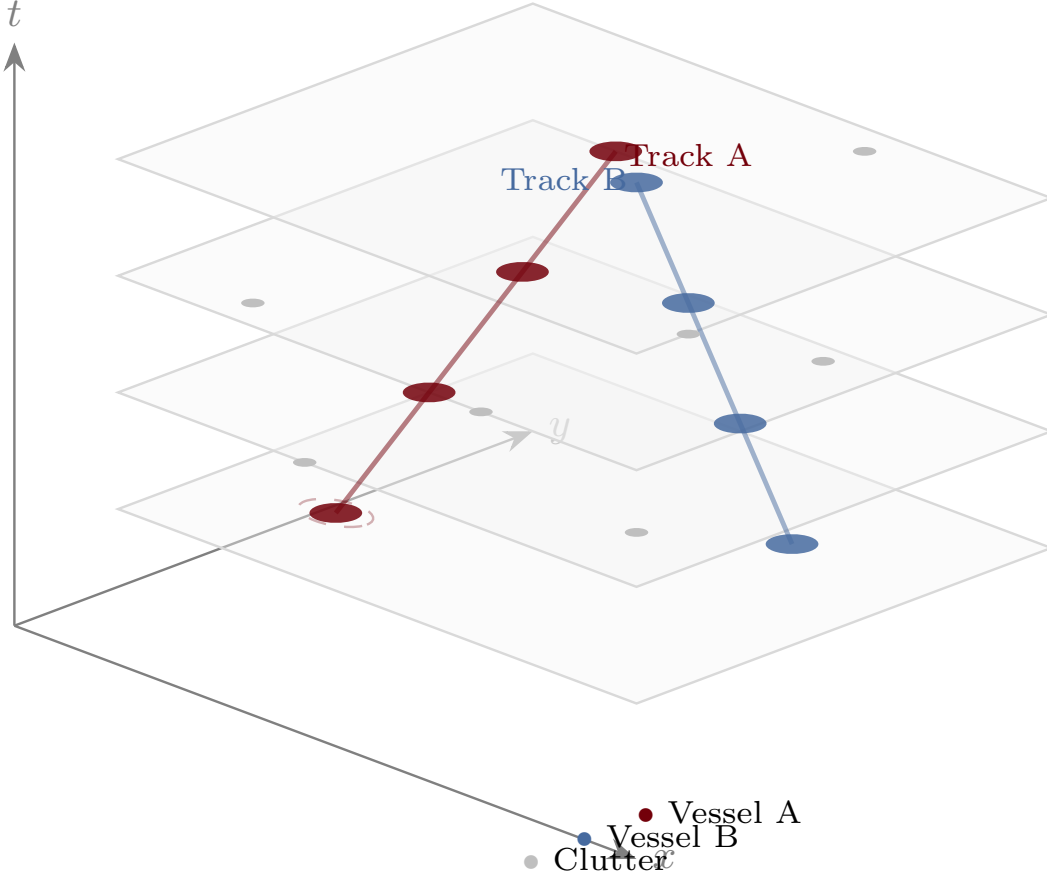
Fig. 5 Spatio-temporal tube visualization. Clusters form connected tubes through the (x, y, t) space, where each tube represents a tracked object trajectory across multiple radar sweeps.
