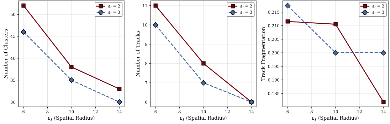
Fig. 12 Sensitivity of tracking metrics to spatial radius \epsilon_s for different temporal radii \epsilon_t . Larger spatial radii produce fewer, larger clusters with reduced fragmentation.
